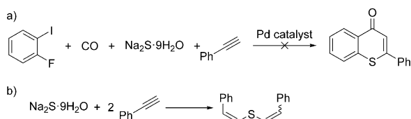
Figure 1. a) Desired thiochromenone synthesis. b) Addition reaction between \text{Na}_2\text{S}\cdot 9\text{H}_2\text{O} and phenyl acetylene.
