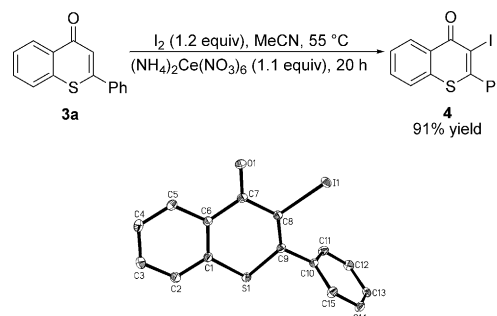
Scheme 2. Top: Synthesis of 3-iodo-2-phenyl-4 H -thiochromen-4-one. The yield is that of isolated 4 . Bottom: Molecular structure of 4 . [22] Hydrogen atoms omitted for clarity.
